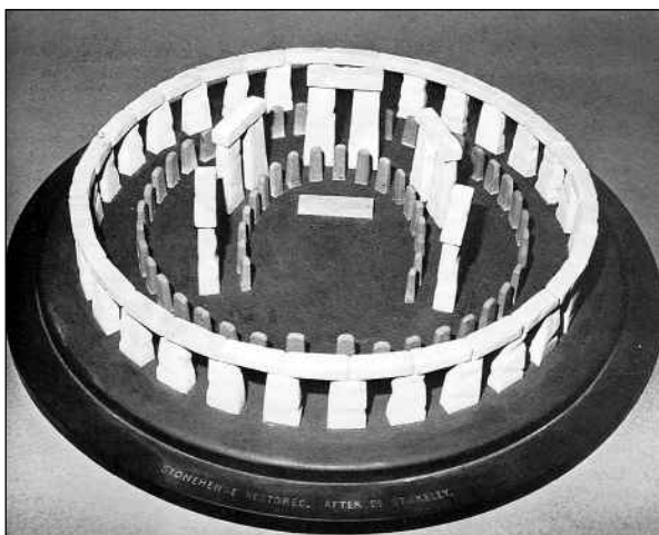
Stonehenge modellje
